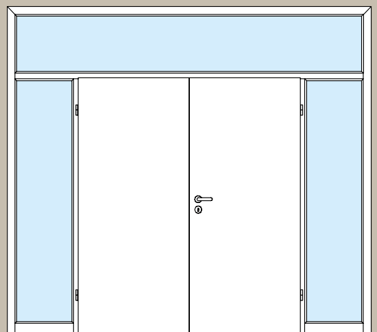
Double-leaf, 2 side elements, 1 transom light
