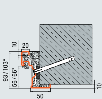
Corner frame with diagonal fixing (Brickwork / unplastered brickwork / concrete)
