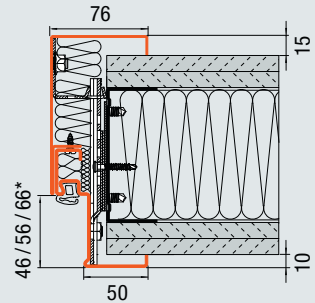
2-part profile frame with concealed plug-and-screw fitting and mineral wool backfilling (partition wall) F90 A and F90 B (shown: F90 A)
