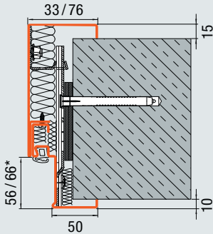
2-part profile frame with concealed plug-and-screw fitting and mineral wool backfilling (Brickwork / unplastered brickwork / concrete, also for plastered brickwork)
