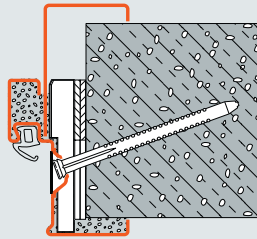
Diagonal fixing With counter frame Vario B53 as a 2-part profile frame (Gas concrete)
