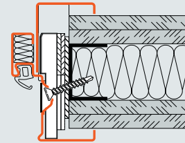
Diagonal fixing With counter frame Vario B53 as a 2-part profile frame (Partition wall F90 A)
