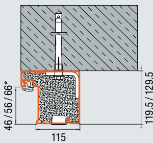
Block frame with flush-fitting cover caps as concealed plug-and-screw fitting in front of the opening (Brickwork / max. T30 doors)
