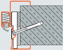
Diagonal fixing With counter frame Vario B53 as a 2-part profile frame (Unplastered brickwork / concrete)
