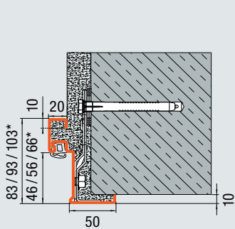
Corner frame with plug-and-screw fitting in the reveal (Brickwork / concrete)
