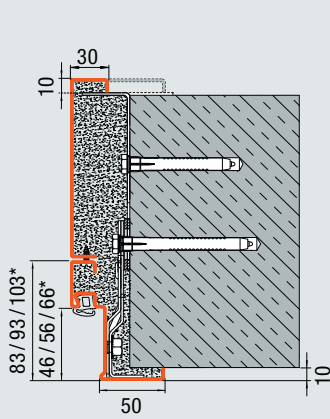
Corner and counter frame with concealed plug-and-screw fitting and counter frame with fitting by welding (Unplastered brickwork / concrete)
