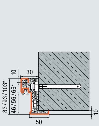
Corner frame with concealed plug-and-screw fitting (Unplastered brickwork / concrete)
