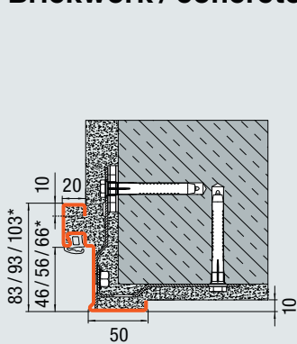
Corner frame with plug-and-screw fitting (Brickwork / concrete)
